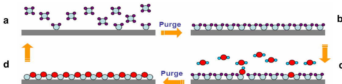
Figure 2: Schematic illustration of the ALD process. Alternating pulses of two different precursors, separated by a purge pulse of an inert gas, constitute a typical ALD cycle. Multiple ALD cycles are used to deposit a film.
